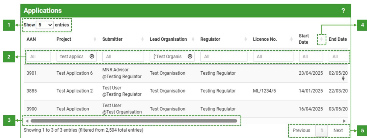
Figure 7. Example view of a MNR table with the different table controls highlighted: 1) a drop-down menu to adjust the number of table entries shown, 2) column header search boxes, 3) a horizontal scroll bar, 4) arrows to sort table columns, and 5) buttons to navigate between pages.
