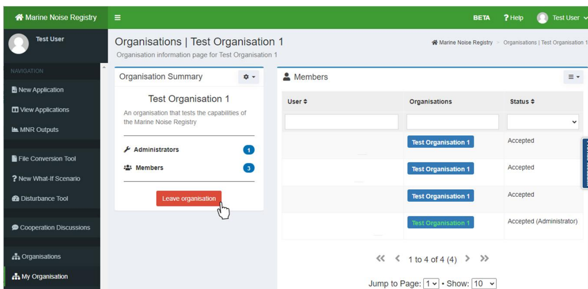
Figure 23. Example of leaving an organisation from the 'My Organisation' page.
