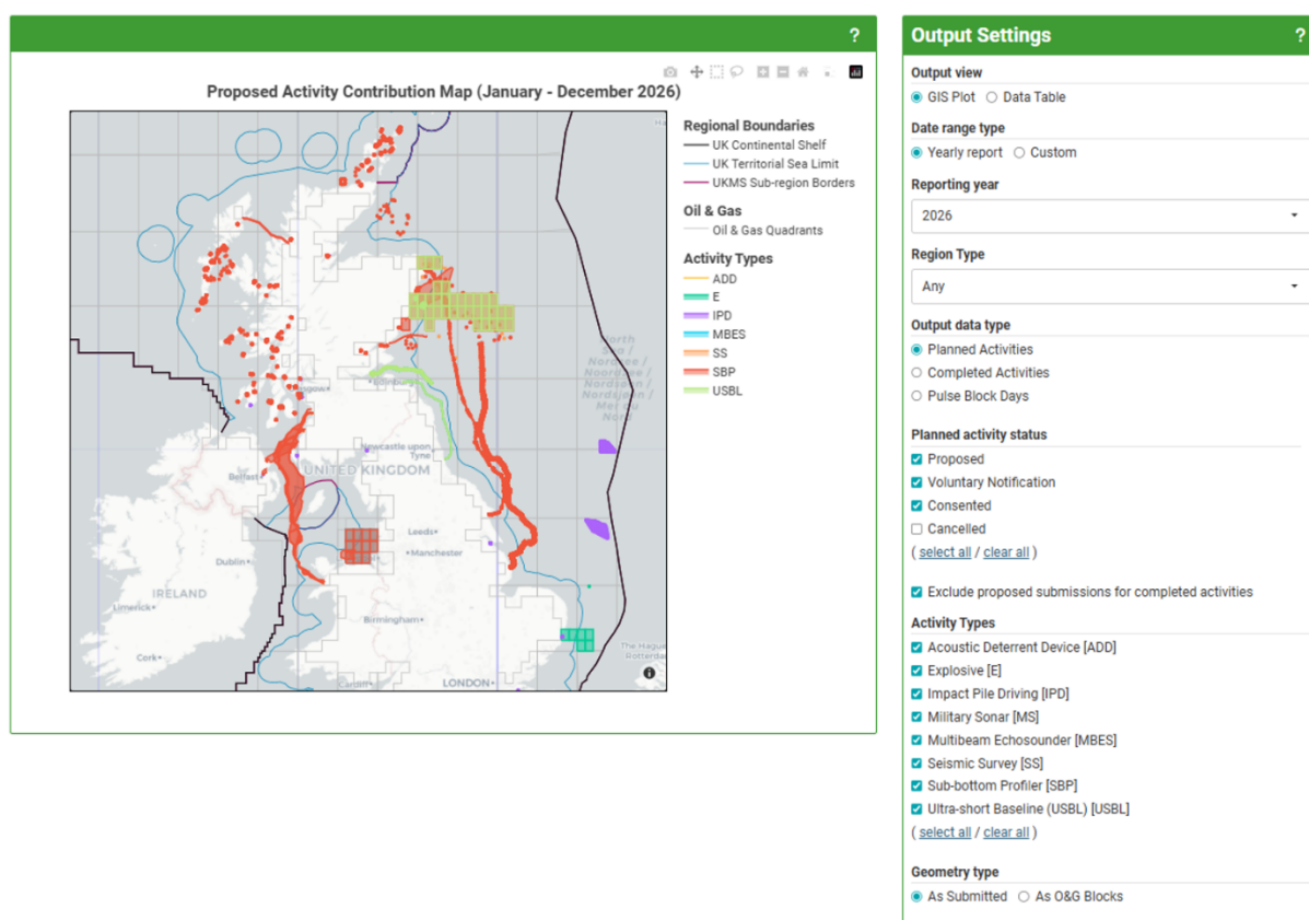
Figure 106. Default view of the 'MNR Outputs' page consisting of a GIS plot (left) and a 'Output Settings' panel (right) allowing users to switch between viewing data as a GIS plot or a data table.
