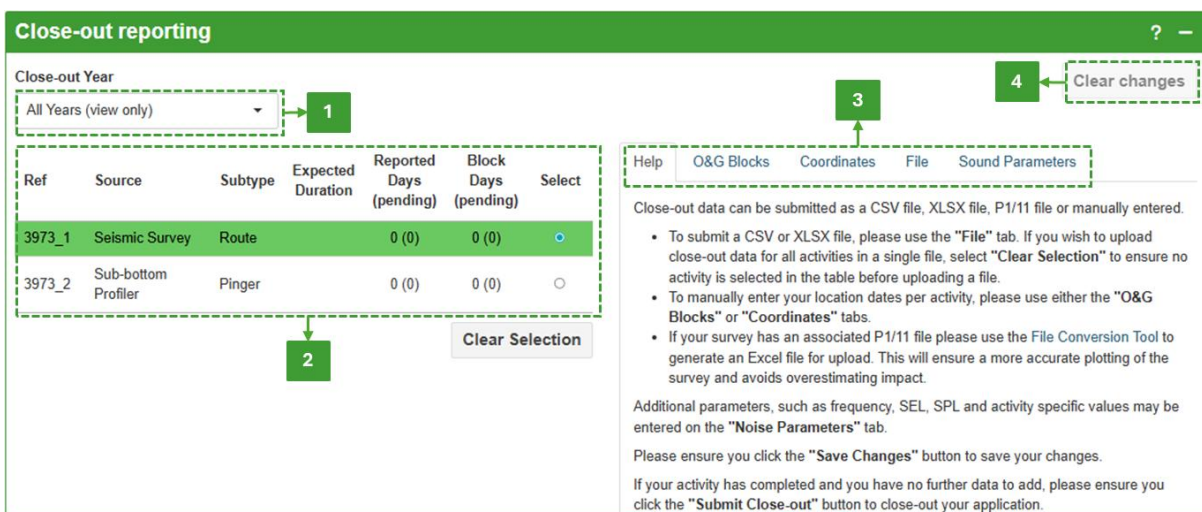
Figure 68. Example view of the 'Close-out Reporting' panel with different components highlighted: 1) a drop-down menu to select which year to view or edit; 2) a table listing all activities of the application; 3) tabs for add locations, dates, and sound parameters to an activity; 4) a button to clear all changes made while editing the panel.
