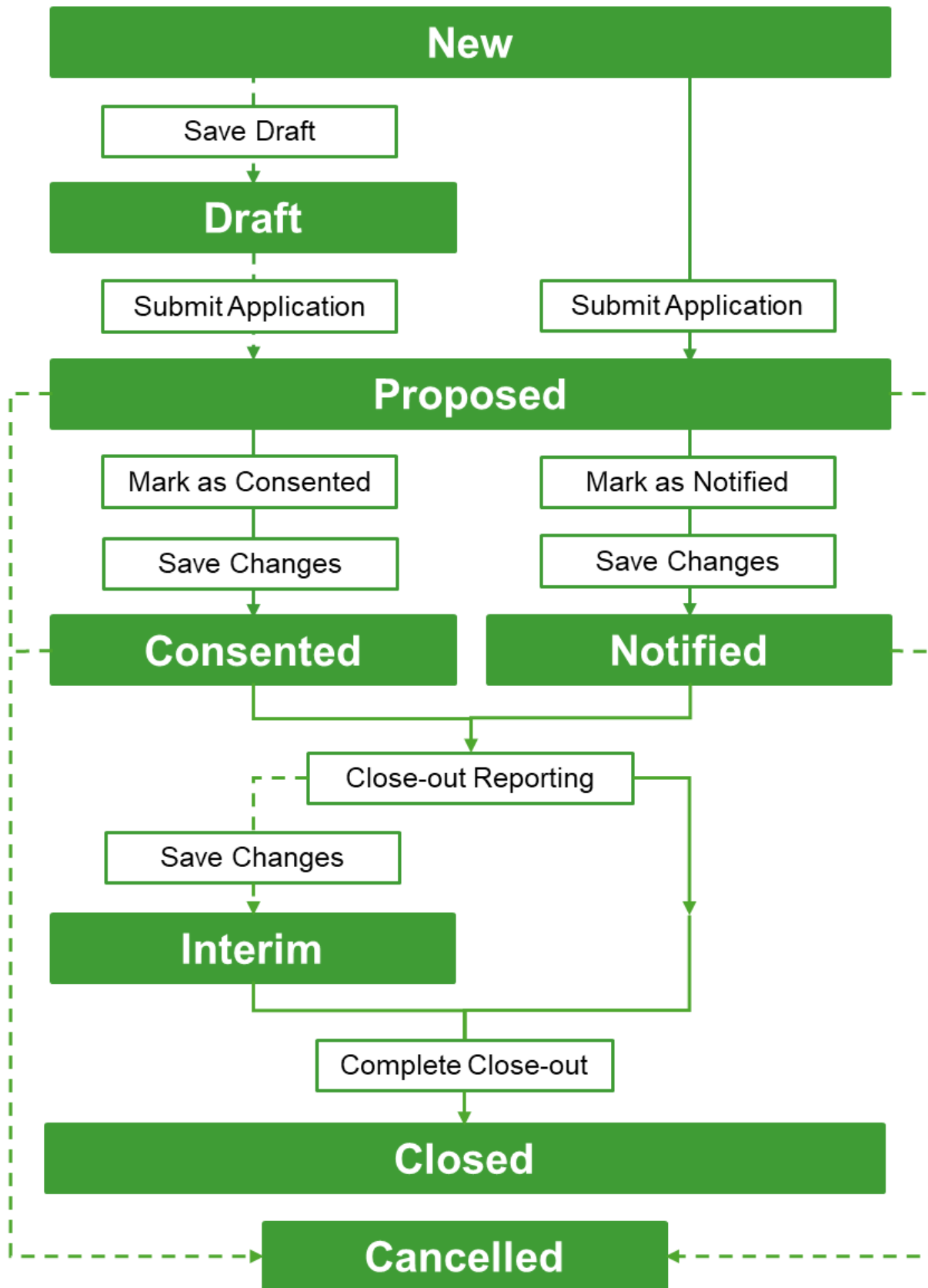
Figure 41. A flow diagram visualising how an application progresses through the MNR. Boxes with a solid fill show different application statuses, boxes with a transparent fill are user actions. Solid lines are mandatory steps; dotted lines are optional actions a user can perform.
